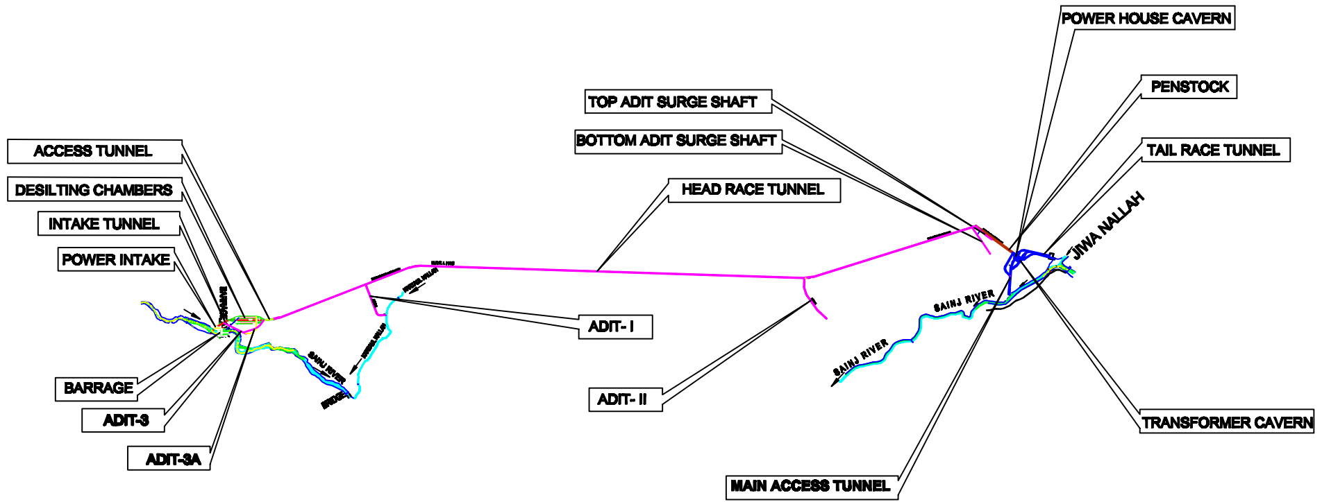
LAYOUT PLAN (NOT TO SCALE)
